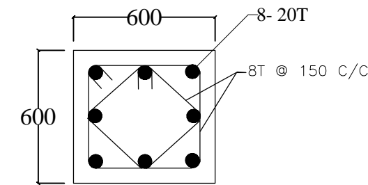
COLUMN DETAIL
