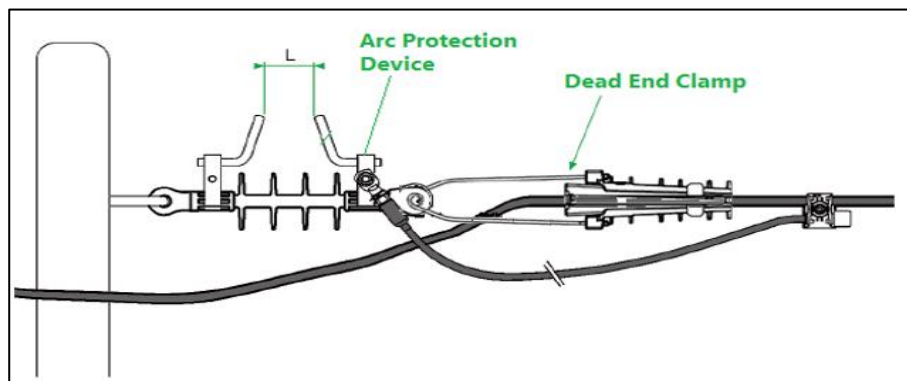
Fig.4:- Arc Protection Device
