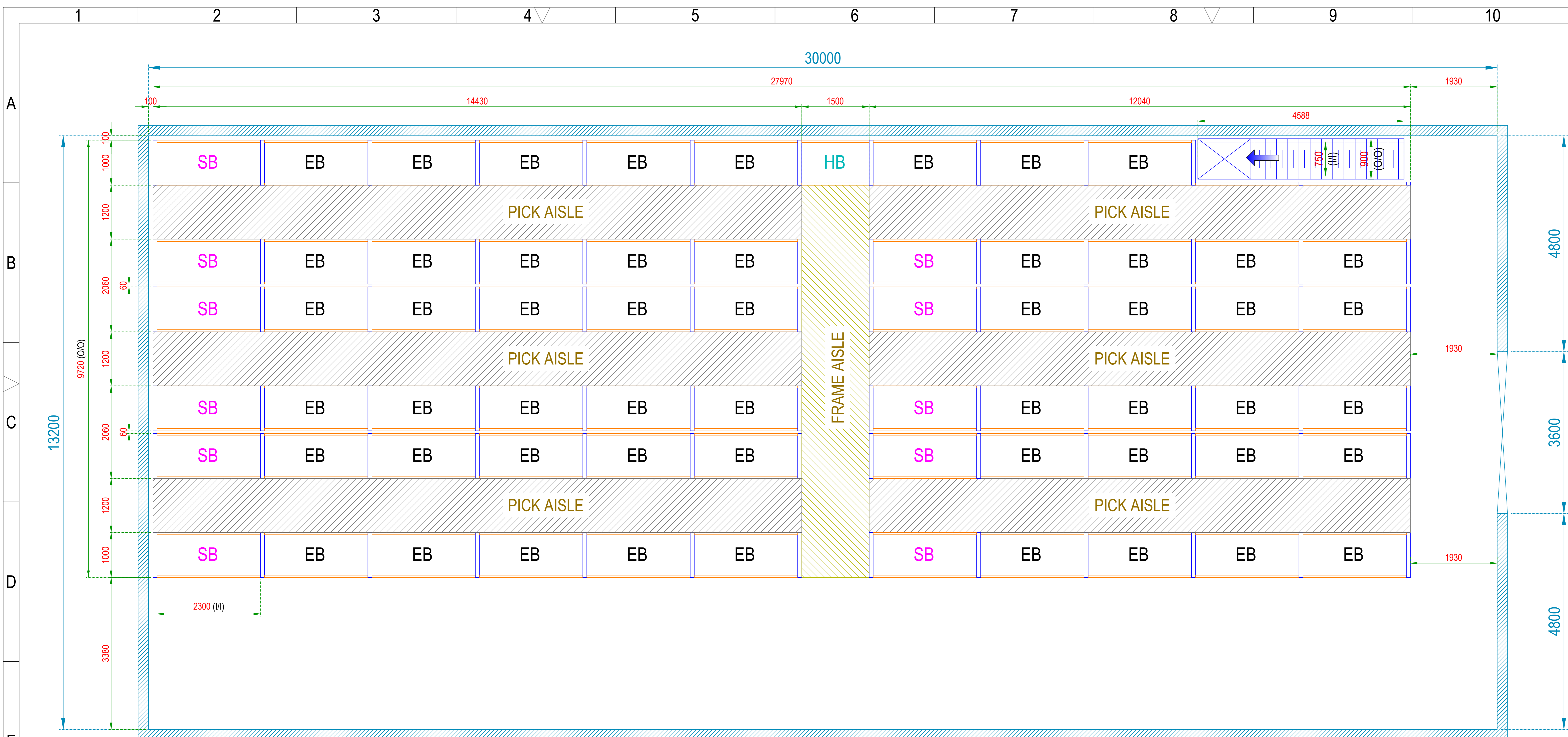
PLAN VIEW OF MTHDS SYSTEM
