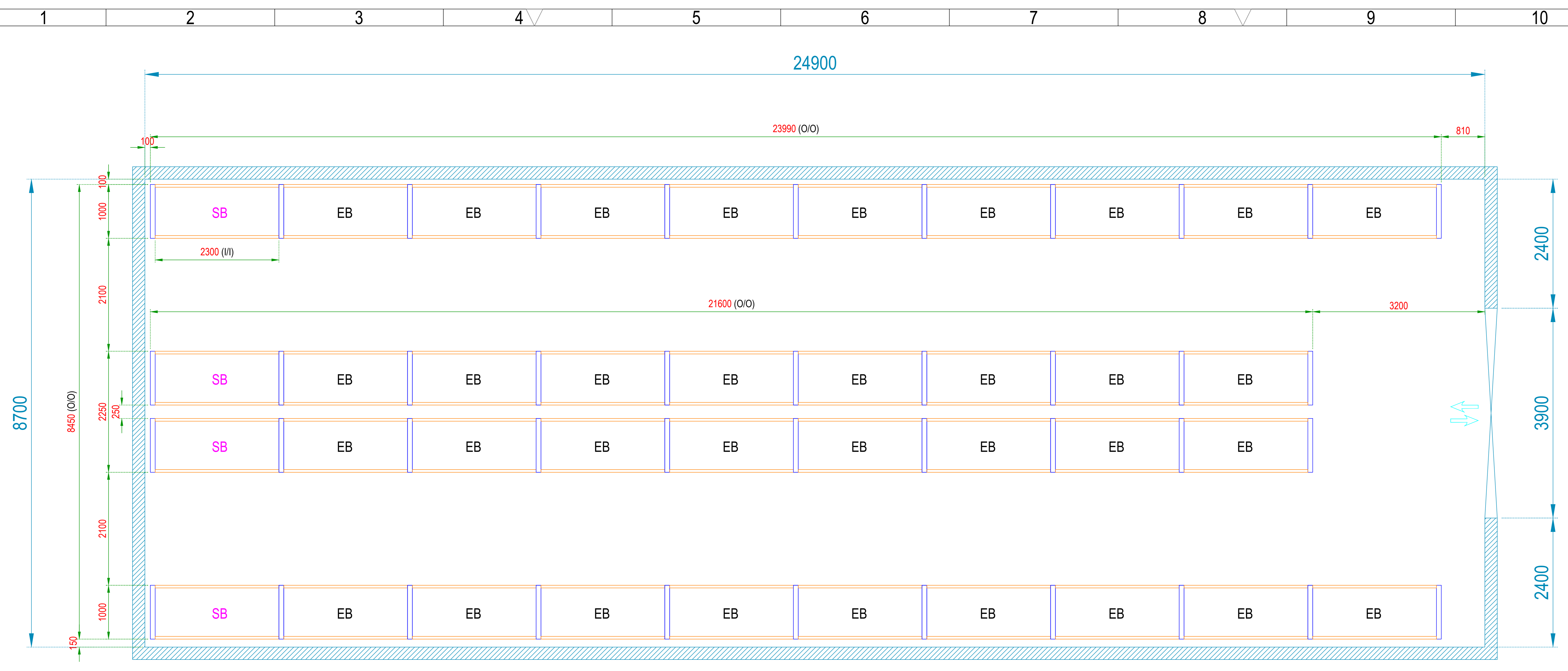
PLAN VIEW OF HDS SYSTEM
