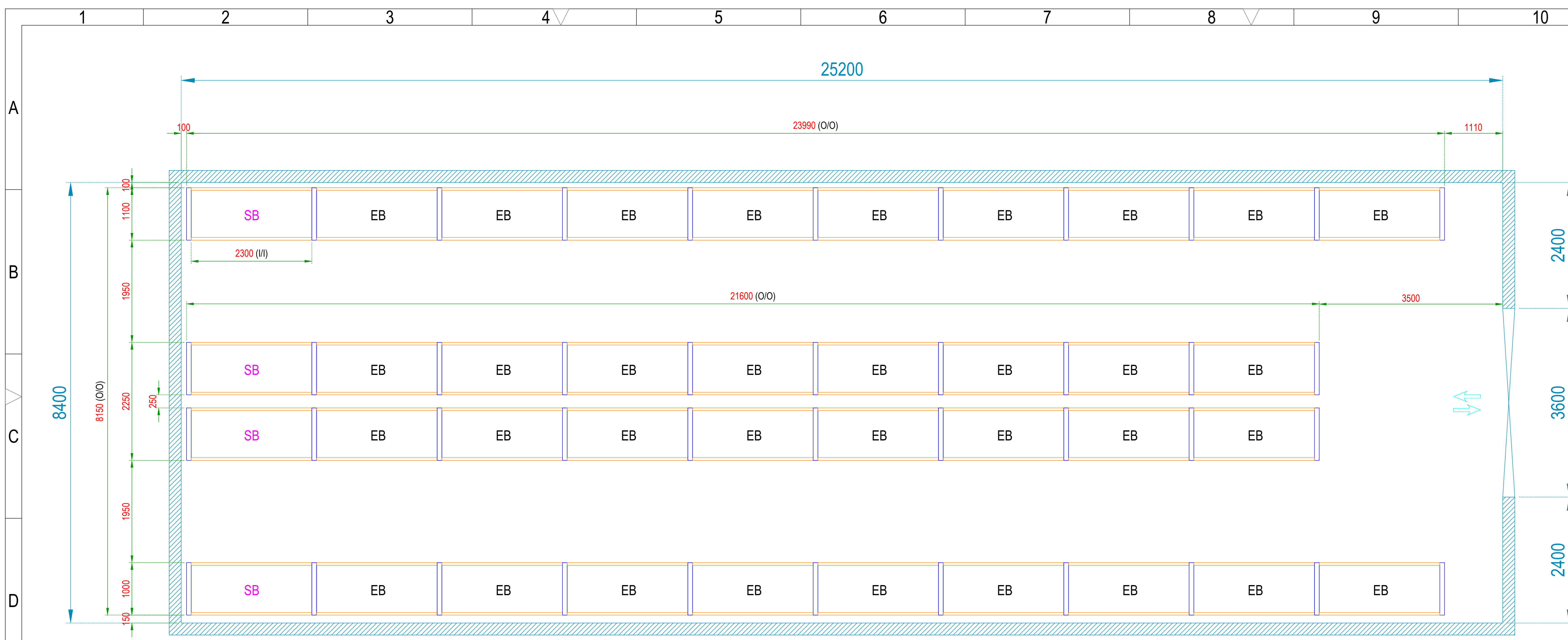
PLAN VIEW OF HDS SYSTEM
