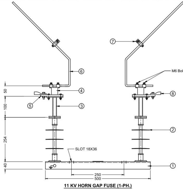
11 KV HORN GAP FUSE (1-PH.)
