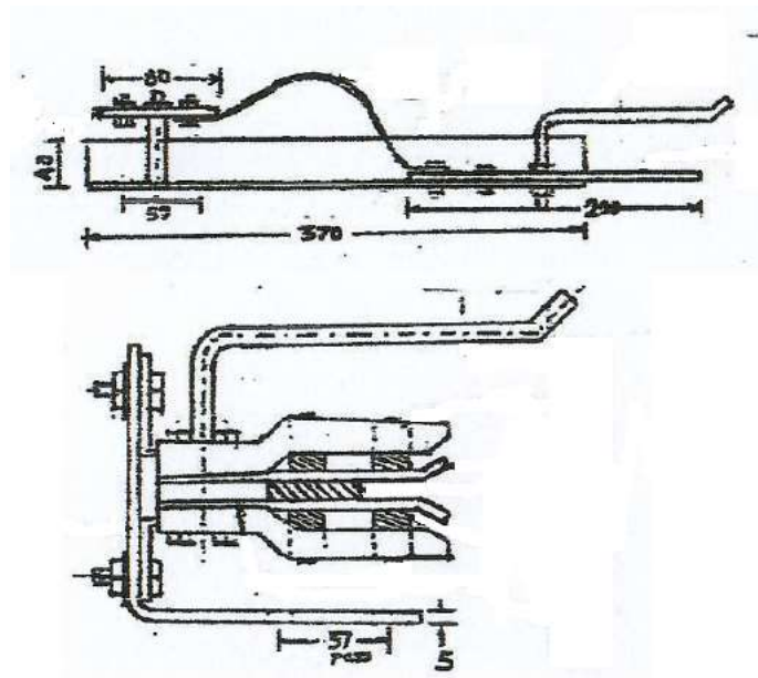
Indicative drawing of Male-Female Contacts Assembly- 11 KV 400A and 200A AB Switch(Horizontal)
