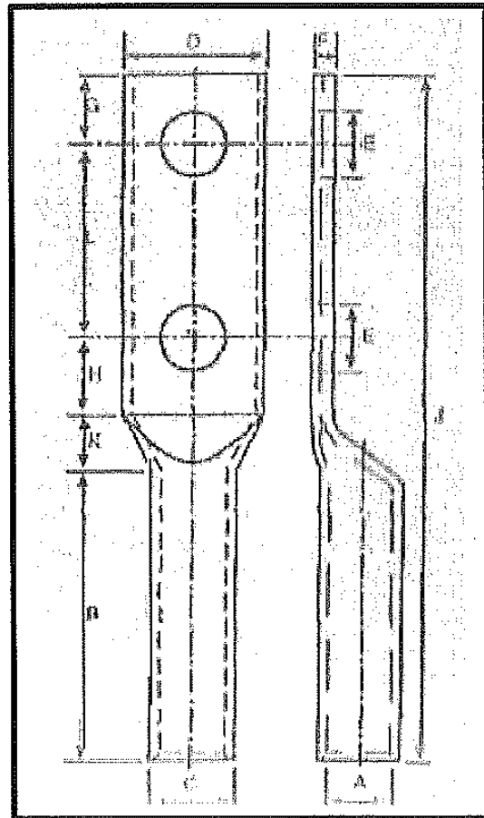
Diagram of Double Hole
