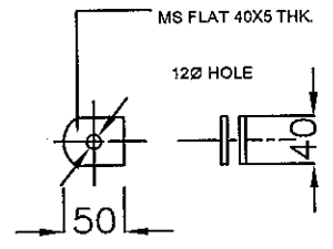
DETAIL - B LOCKING ARRANGEMENT
