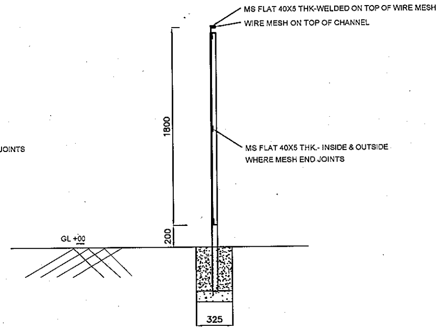
SECTIONAL ELEVATION - BB'
