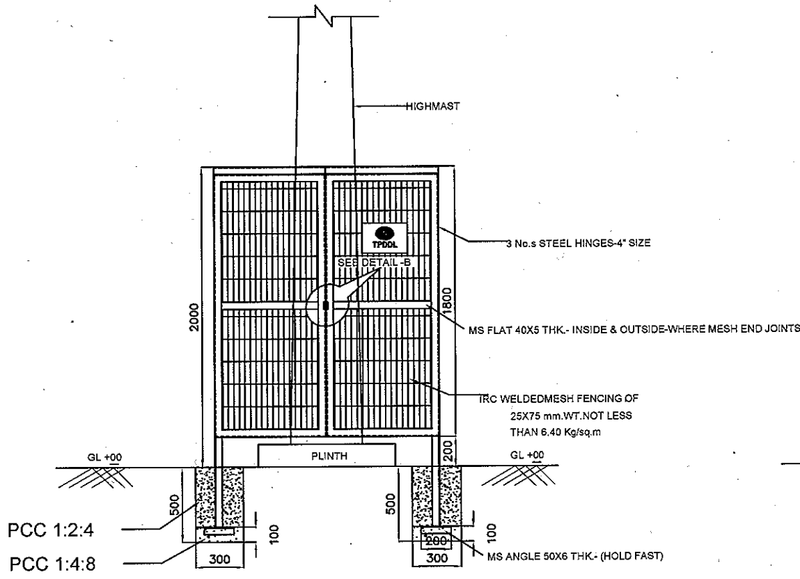
ELEVATION - A - A'
